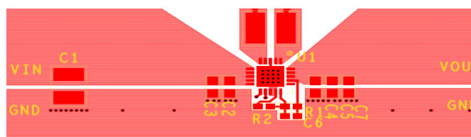
FIGURE 23. RECOMMENDED LAYOUT
