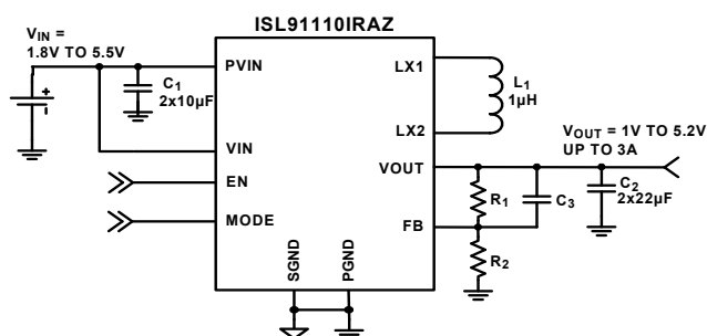
FIGURE 22. ADJUSTABLE OUTPUT APPLICATION
