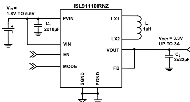
FIGURE 1. TYPICAL APPLICATION: V_{OUT} = 3.3V
