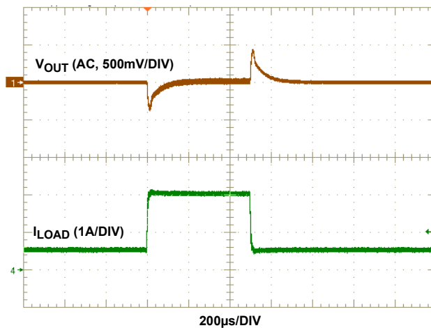
FIGURE 20. 0.5A TO 2A LOAD TRANSIENT ( V_{IN} = 3.6\text{V} , V_{OUT} = 5\text{V} )
